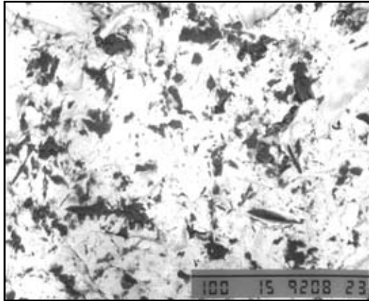
Figure 1. Medium power scanning electron micrograph (backscattered electron imaging mode) of a bA surface showing the blast-induced roughness and embedded blast residue as dark inclusions in the surface. Bar=100 \mu m.
