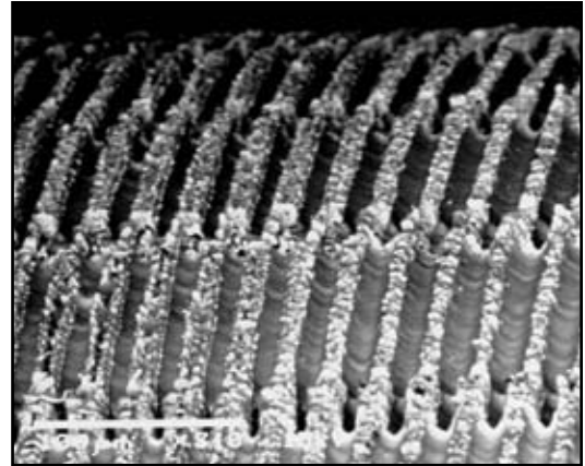
Figure 2. Medium power scanning electron micrograph of a prototype dental implant with the upper 1 mm of the collar microtextured with the MG12 surface. Bar=100 \mu m. (From Ricci et al., in Bone Engineering , ed. JE Davies, Em 2 Inc. Toronto, Ont. Canada, 2000 reprinted with permission.
